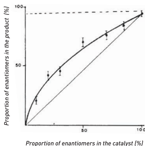
Figure 5. Diagram taken from J. Am. Chem. Soc. 1986, 108, 2353–2357
